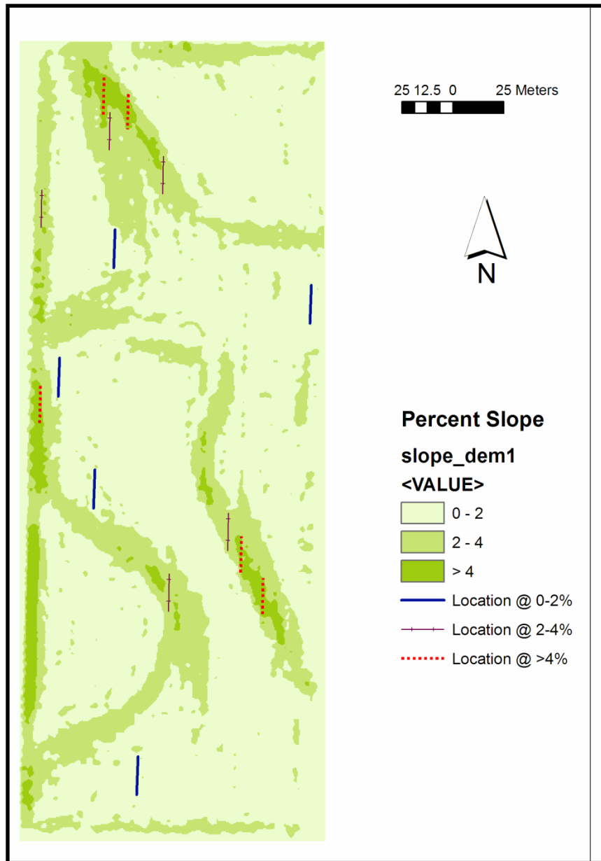
Figure 1. Illustration of slope across the test site represented as percent rise, including sampling locations according to slope category.
