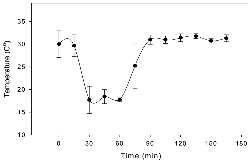
Figure 1. Increase in filter paper temperature as drying occurs.
